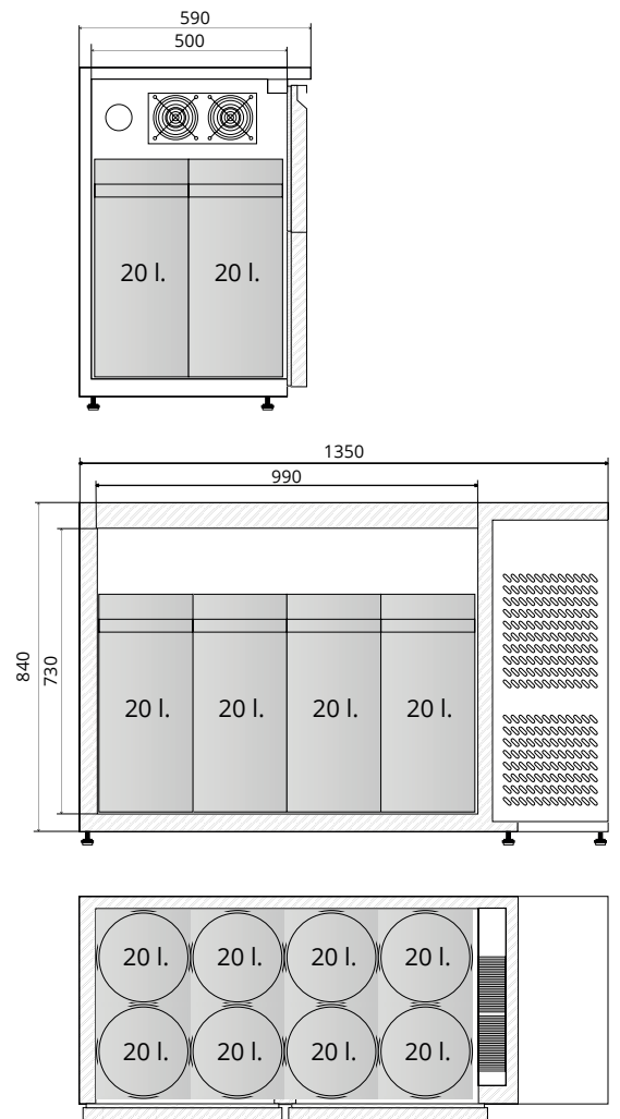
bokorys CKC8 KEG
